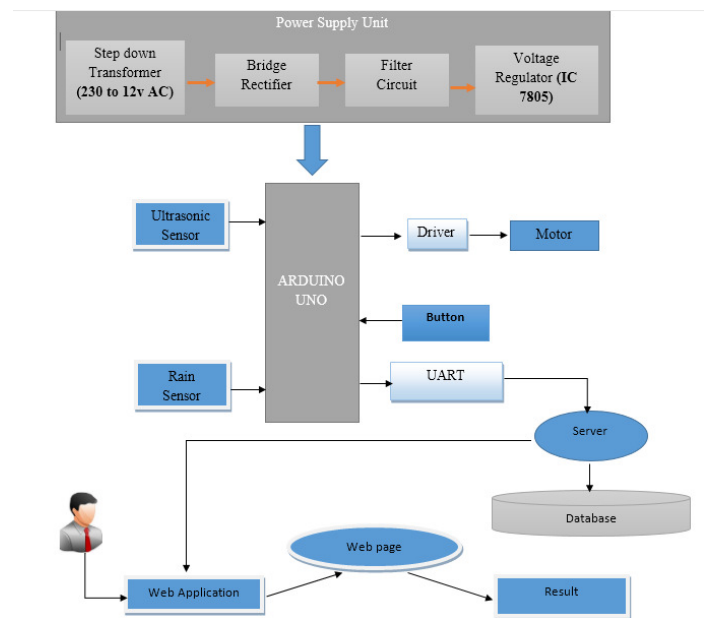
Figure 1 Architecture design
